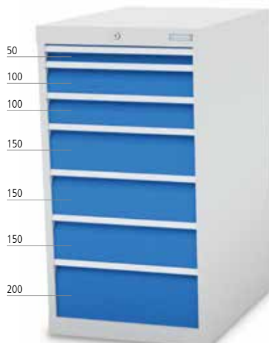
■ 7 x drawer
