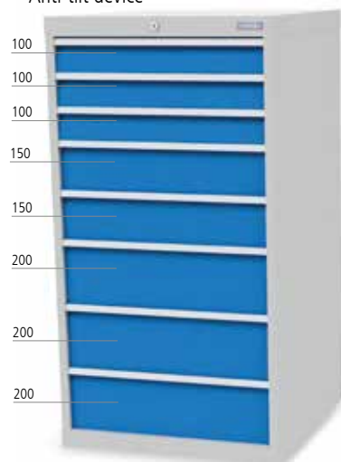
■ 8 x drawer
