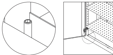
4 adjustable leveling feet, accessible from above with an Allen key (size SW6)
